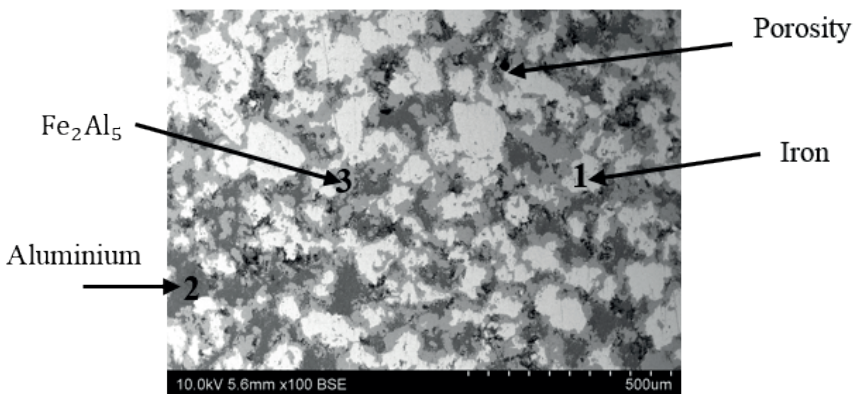
Fig. 6. Microstructure of Al-Fe material centrifuged 20 min and sintered – middle part of the samples (SEM)
