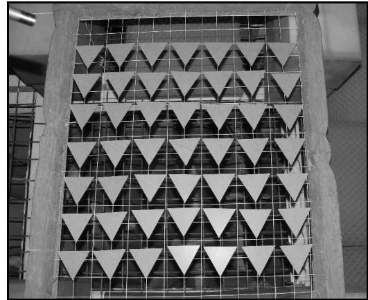
Fig. 13. Array of triangular panels. \mu = 0.37 , \varepsilon = 75.31
