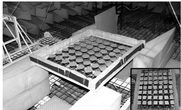
Fig. 15. Array of circles ( \mu = 0.44 , \varepsilon = 53.33 ) and squares ( \mu = 0.49 , \varepsilon = 57.17 )
