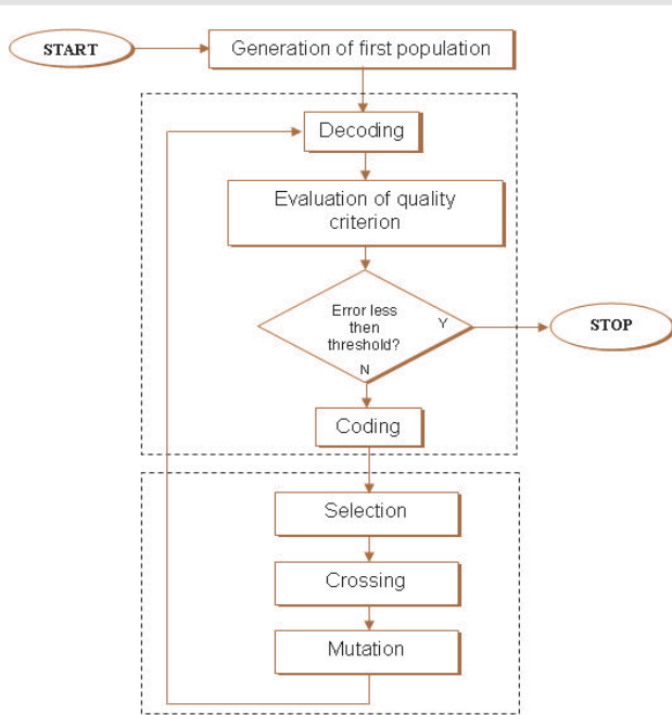
Fig. 1. Step by step workflow
