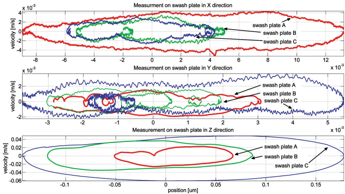
Fig. 6. Phase trajectory runs estimated for different swash plate surfaces in X , Y , Z direction – transducers mounted on swash plate
