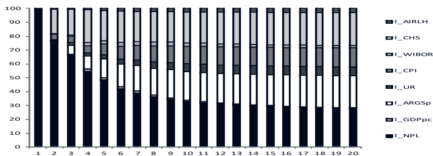
Figure 7. Forecast variance decomposition for I_NPL
