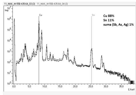
Fig. 3. Bronze sickle, Mogiła (Site 55), 1300 BC: a) the view, b) the X-ray spectrum with identification lines for copper and tin. Concentration of elements: copper – 88%; tin – 11%; sum of admixtures – 1%
