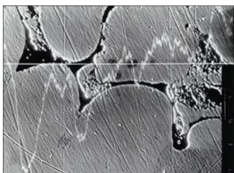
Fig. 5. Scanning image COMPO of inclusions in a sample of silicon bronze CuSi3Zn3MnFe ingots metallurgical illustrating the linear distribution of Fe (magn. 1000x)
