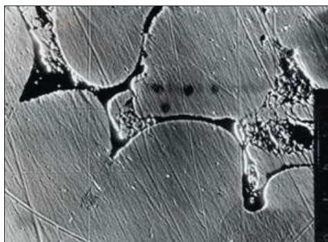
Fig. 4. Scanning image COMPO of inclusions in a sample of silicon bronze CuSi3Zn3MnFe ingots metallurgical (magn. 1000x)
