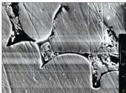
Fig. 1. Scanning image SEI of inclusions in a sample of silicon bronze CuSi3Zn3MnFe ingots metallurgical (magn. 1000x)
