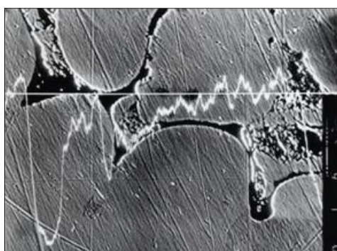
Fig. 6. Scanning image COMPO of inclusions in a sample of silicon bronze CuSi3Zn3MnFe ingots metallurgical illustrating the linear distribution of Mn (magn. 1000x)
