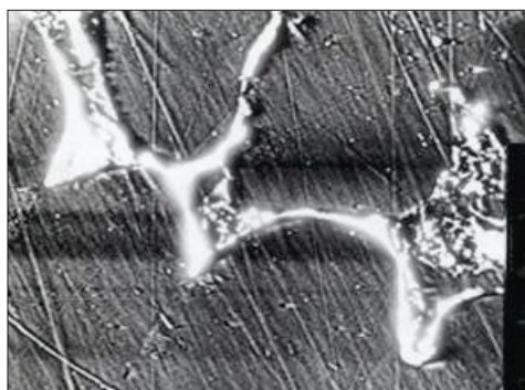
Fig. 2. Scanning image AEI of inclusions in a sample of silicon bronze CuSi3Zn3MnFe ingots metallurgical (magn. 1000x)
