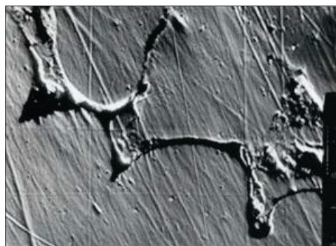
Fig. 3. Scanning image TOPO of inclusions in a sample of silicon bronze CuSi3Zn3MnFe ingots metallurgical (magn. 1000x)
