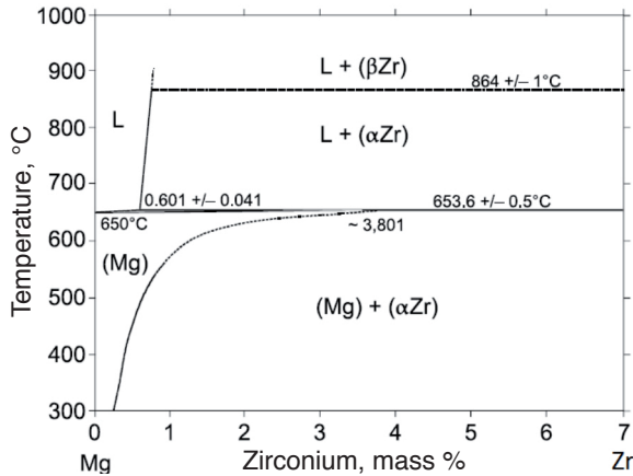
Fig. 6. Phase diagram of Mg-Zr system [1]
