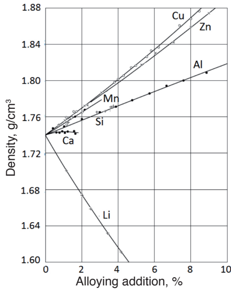
Fig. 2. Influence of alloying elements on the density of magnesium at room temperature [1]
