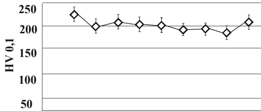
Fig. 4. HV 0.1 genuine material microhardness research
