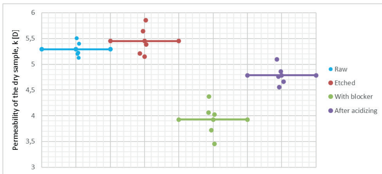
Fig. 10. Average permeability of samples at each stage of the study
