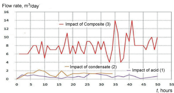
Fig. 3. Comparison of the flow rate of oil well H-1 after alternating exposure to the clogged bed of acid (1), condensate (2) and Composite (3)
