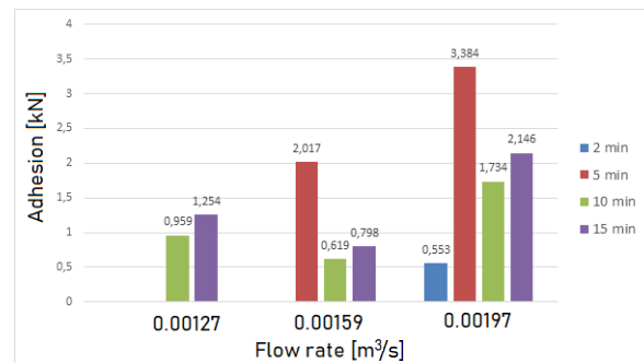
Fig. 6. Average values of adhesion for various pumping rates of the washing fluid and for various washing times
