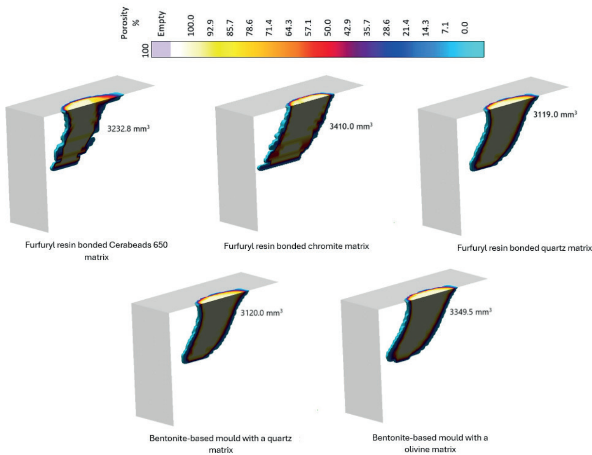
Fig. 6. Change in the shape of shrinkage porosity depending on the used molding material
