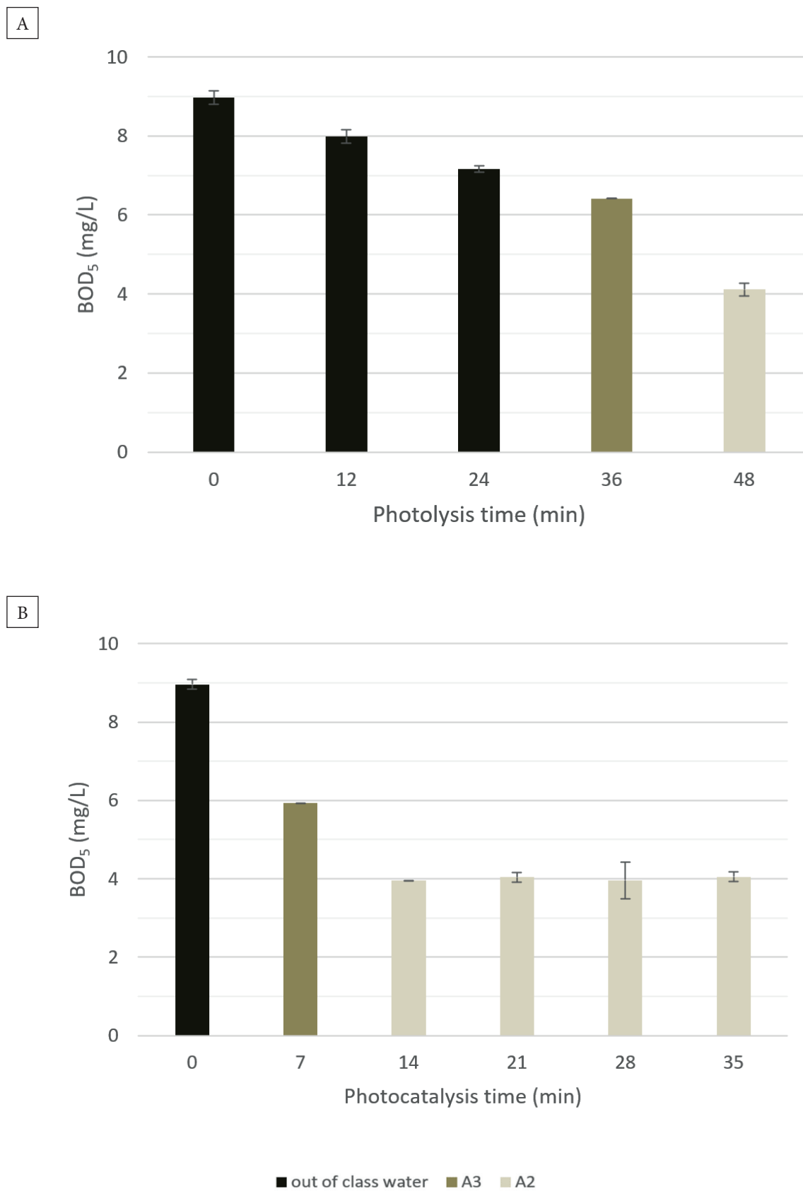
Fig. 2. Variations of BOD over time during UV photolysis (A) and UV photocatalysis with TiO 2 -MMT catalyst (B) with the assignment of water quality categories
