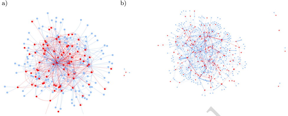
Figure 1. User-relationship-distribution comparison: a) user relationships on DAR data set; b) user relationships on CG data set.
