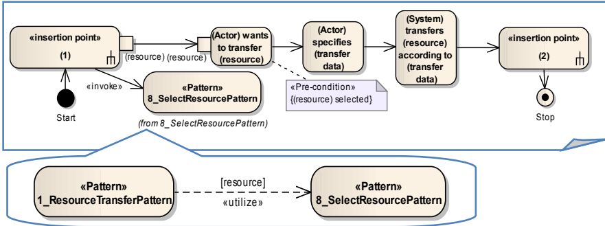
Figure 4. Insertion of application logic “snippet” into flow of interaction describing other functionality.
