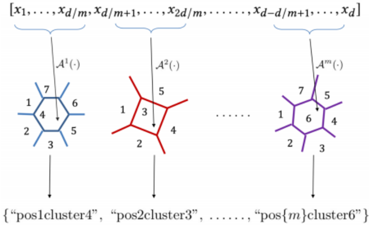
Figure 4. Illustration of subvector-wise clustering
