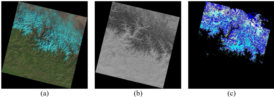
Figure 6. Landsat 8 OLI/TIRS C1 level-2 images of Indian Himalayan region: a) natural color image; b) thermal image of the same region in (a); c) quality region image of the same region in (a)
