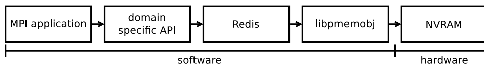
Figure 2. Technology stack used for testing. MPI application calls domain-specific API – abstract layer that covers Redis. Redis uses NVRAM as its persistent storage.
