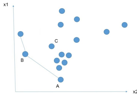
Figure 3. Illustration of a classification problem based on minimizing x_1 and x_2 criteria. Connected points form a Pareto front.
