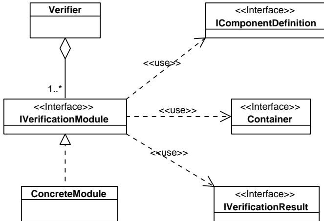
Figure 4. Verifier modules UML scheme.
