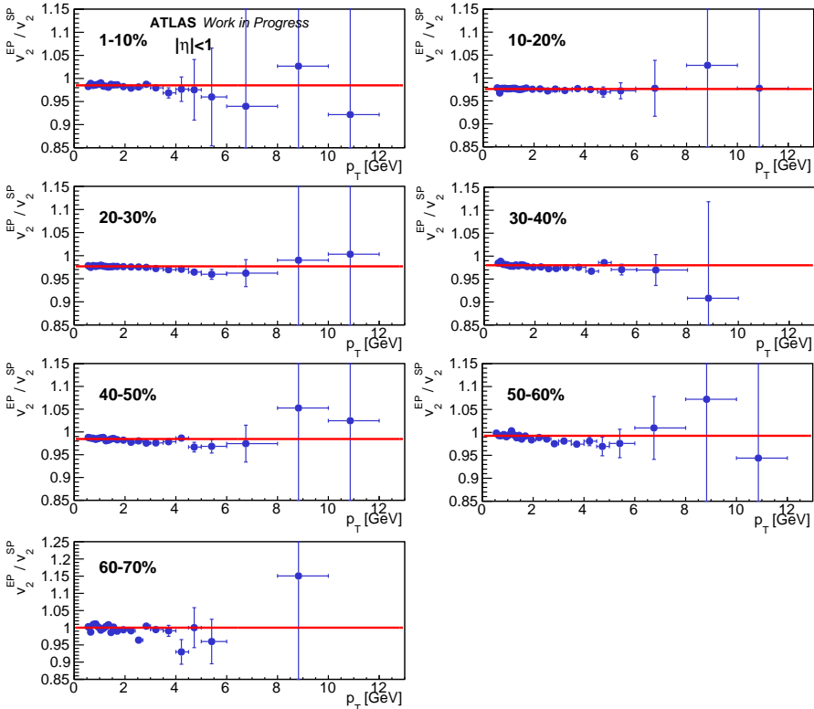
Figure 8. Ratios of elliptic flow coefficients, v_2^{\text{EP}}/v_2^{\text{SP}} , measured with the EP and SP methods as a function of p_T in different centrality classes. A constant (red line) is a fit to the points.
